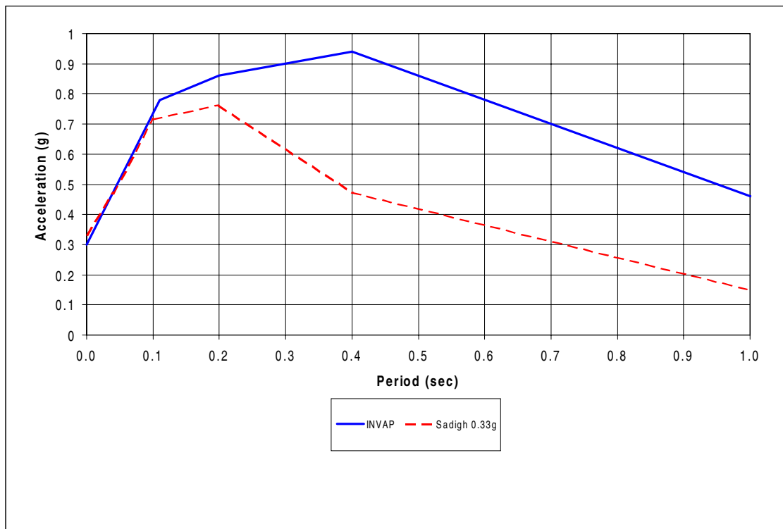
Figure 1 – Comparison between design value and disaggregated IGNS value.
