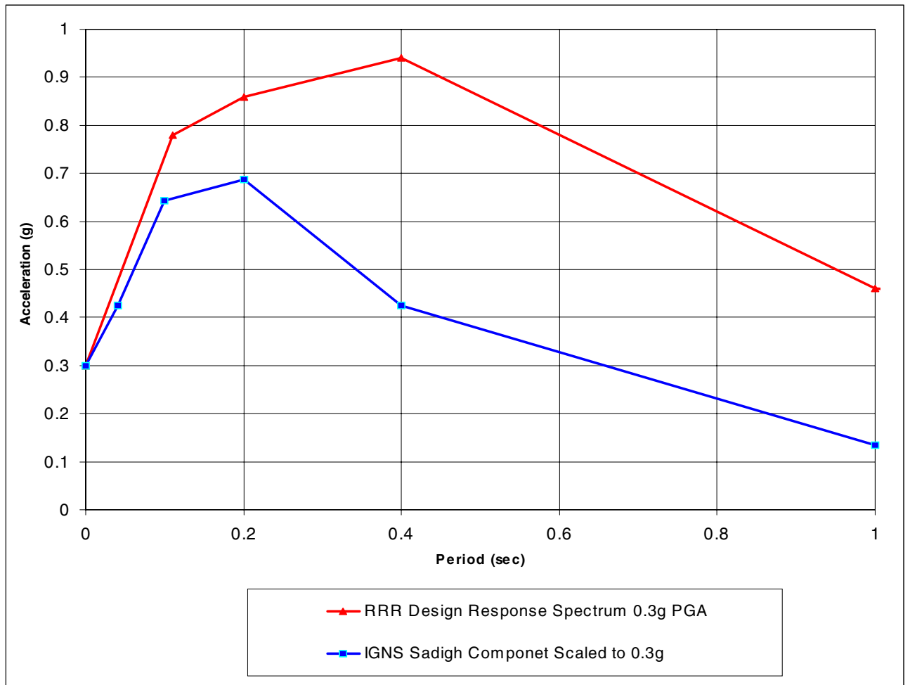
Figure 2 – Comparison between design value and reduced IGNS value.
