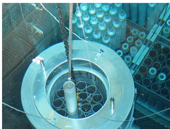
Figure 7: Wet storage facility used for former HIFAR reactor spent fuel
