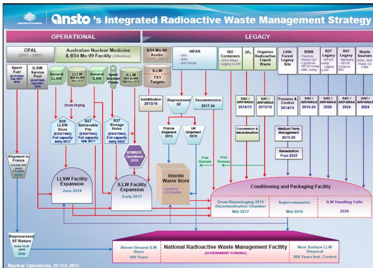
Figure 4: ANSTO's integrated radioactive waste management strategy for LLW and ILW.
